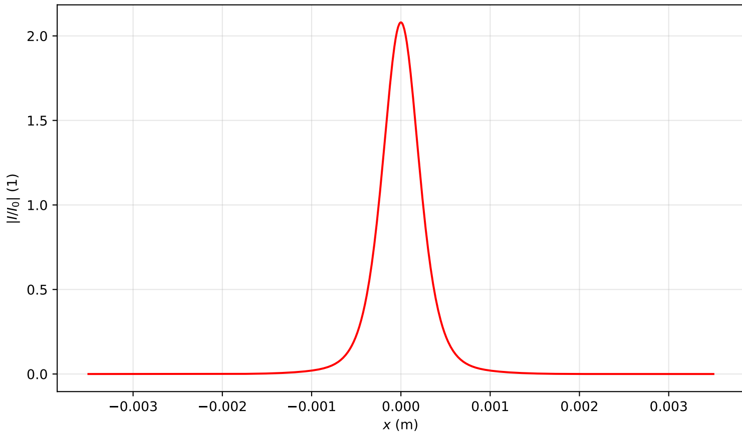
Intensity profile I(x, y = 0, z = 1.911)/I_0 , P_{in}=1.0P_{cr} , artificial time
